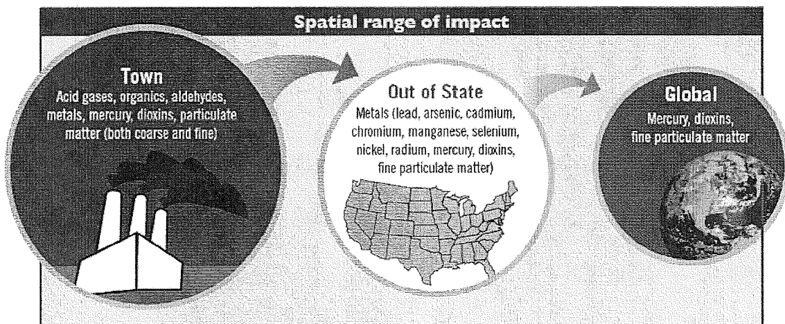
Figure 9. Schematic of the likely range that hazardous air pollutants are transported.
