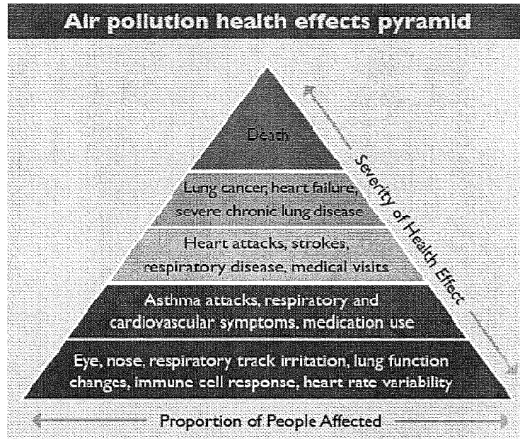
Figure 8. Air Pollution Health Effects Pyramid.
