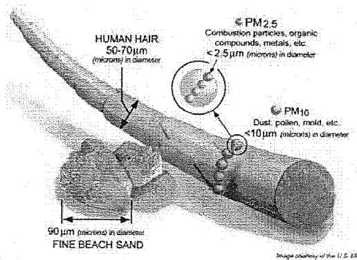
Figure 7. Fine PM: Aerosols Smaller than 2.5 microns Across ( PM_{2.5} ), Compared with a Human Hair and a Grain of Sand. (EPA Office of Research and Development, http://www.epa.gov/ord/ca/quick-finder/particulate-matter.htm )
