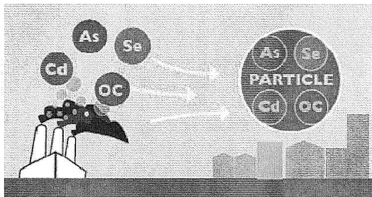
As-Arsenic Cd-Cadmium Se-Selenium OC-Organic Compounds
