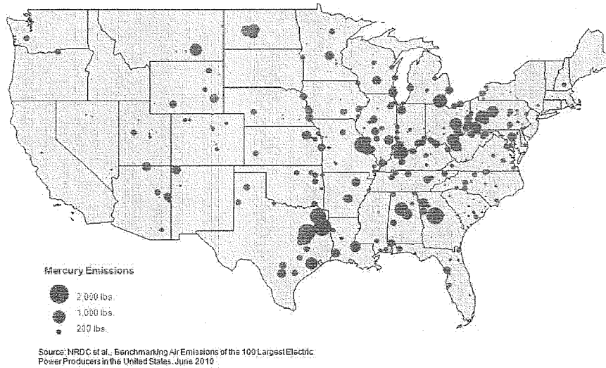
Panel A: Location and Size of US Power Plants by Mercury Emissions
