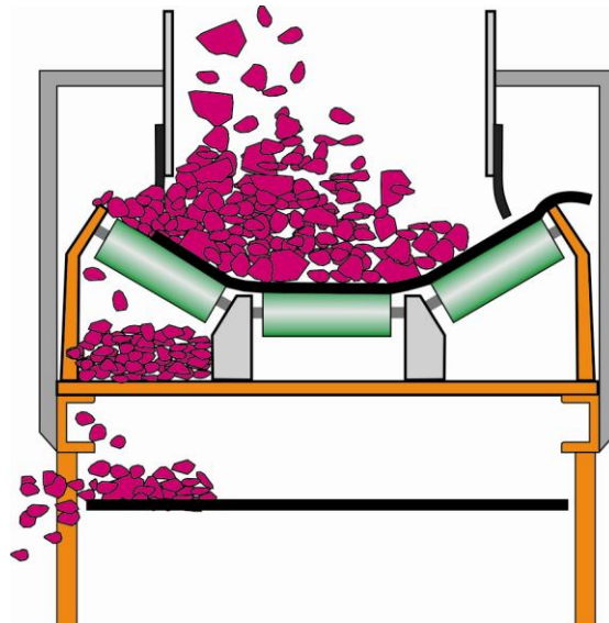
Figure 5.6. Spillage as a result of material being improperly fed onto a belt.
