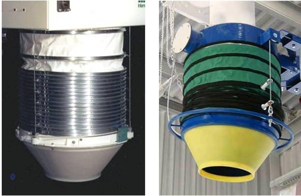
Figure 7.2. Loading spout discharge cones designed to seal against the loading port of closed vehicles to minimize dust liberation.
