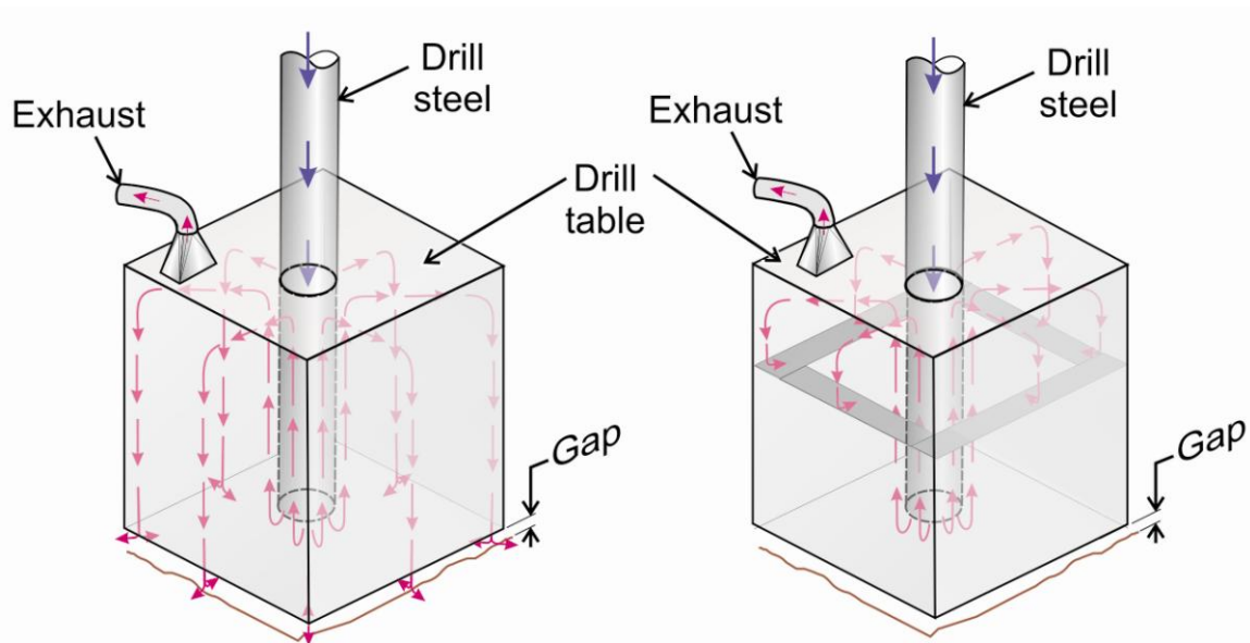
Figure 3.9. Qualitative models of airflow patterns underneath the shroud without the air-blocking shelf (left) and with the air-blocking shelf (right).
