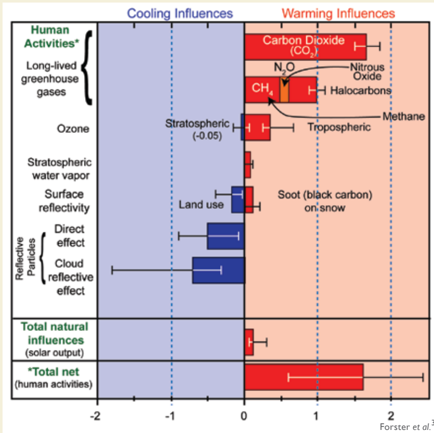
The figure above shows the amount of warming influence (red bars) or cooling influence (blue bars) that different factors have had on Earth's climate over the industrial age (from about 1750 to the present). Results are in watts per square meter. The longer the bar, the greater the influence on climate. The top part of the box includes all the major human-induced factors, while the second part of the box includes the Sun, the only major natural factor with a long-term effect on climate. The cooling effect of individual volcanoes is also natural, but is relatively short-lived (2 to 3 years), thus their influence is not included in this figure. The bottom part of the box shows that the total net effect (warming influences minus cooling influences) of human activities is a strong warming influence. The thin lines on each bar provide an estimate of the range of uncertainty.
