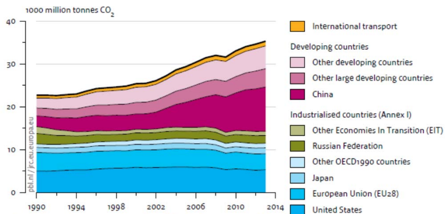
Global CO 2 emissions per region from fossil-fuel use and cement production
